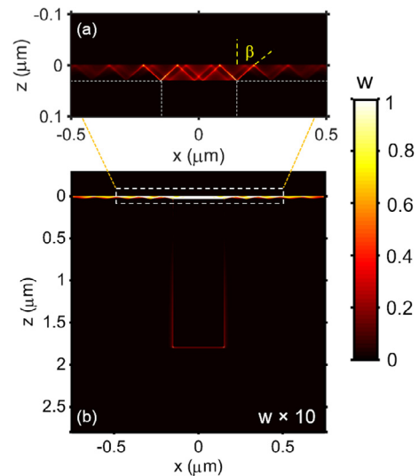
Fig. 8. Local power dissipation density at \nu = 1436 \text{ cm}^{-1} corresponding to the perfect-absorptance peak in Fig. 6(a): (a) zoomed-in profile showing the details inside the hBN film, (b) the dissipation profile (enlarged by one order of magnitude) of the structure. The scale bar for w is in \text{MW}/\text{m}^3 with an upper limit 1 \text{ MW}/\text{m}^3 , beyond which w is displayed with white color. Note that the x and z scales are readjusted to show the profile clearly but the propagation angle \beta is distorted.
